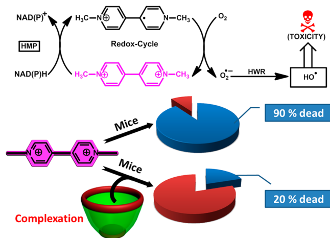
Scheme 5. Biochemical Mechanism of Viologen Toxicity and Detoxification by Complexation with SC5A (HWR, Haber-Weiss reaction; HMP, hexose monophosphate pathway)
