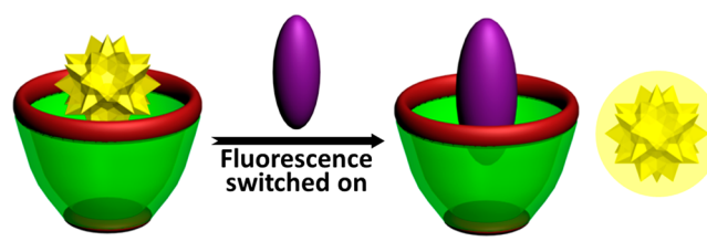
Scheme 2. Analyte Sensing by Dye Displacement
