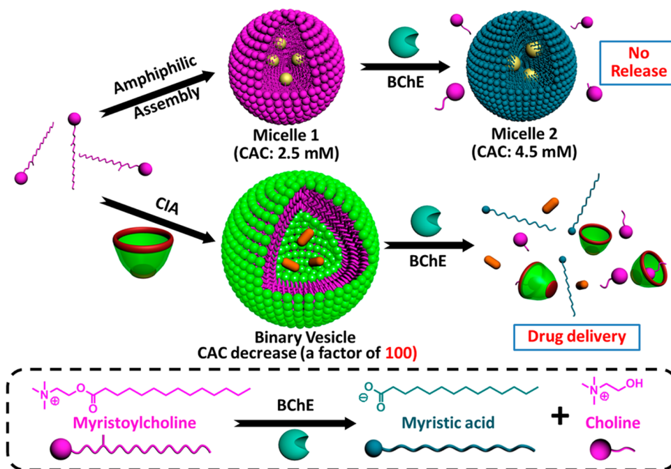
Scheme 10. Enzymatic Responsiveness of Amphiphilic Assemblies of Myristoylcholine Fabricated in the Absence or Presence of SC4A
