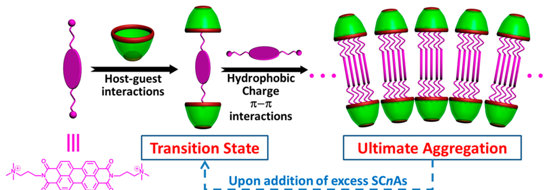
Scheme 8. Construction of SC5A+PMA Supramolecular Binary Vesicles and Temperature-Responsive Drug Release from the Vesicles
