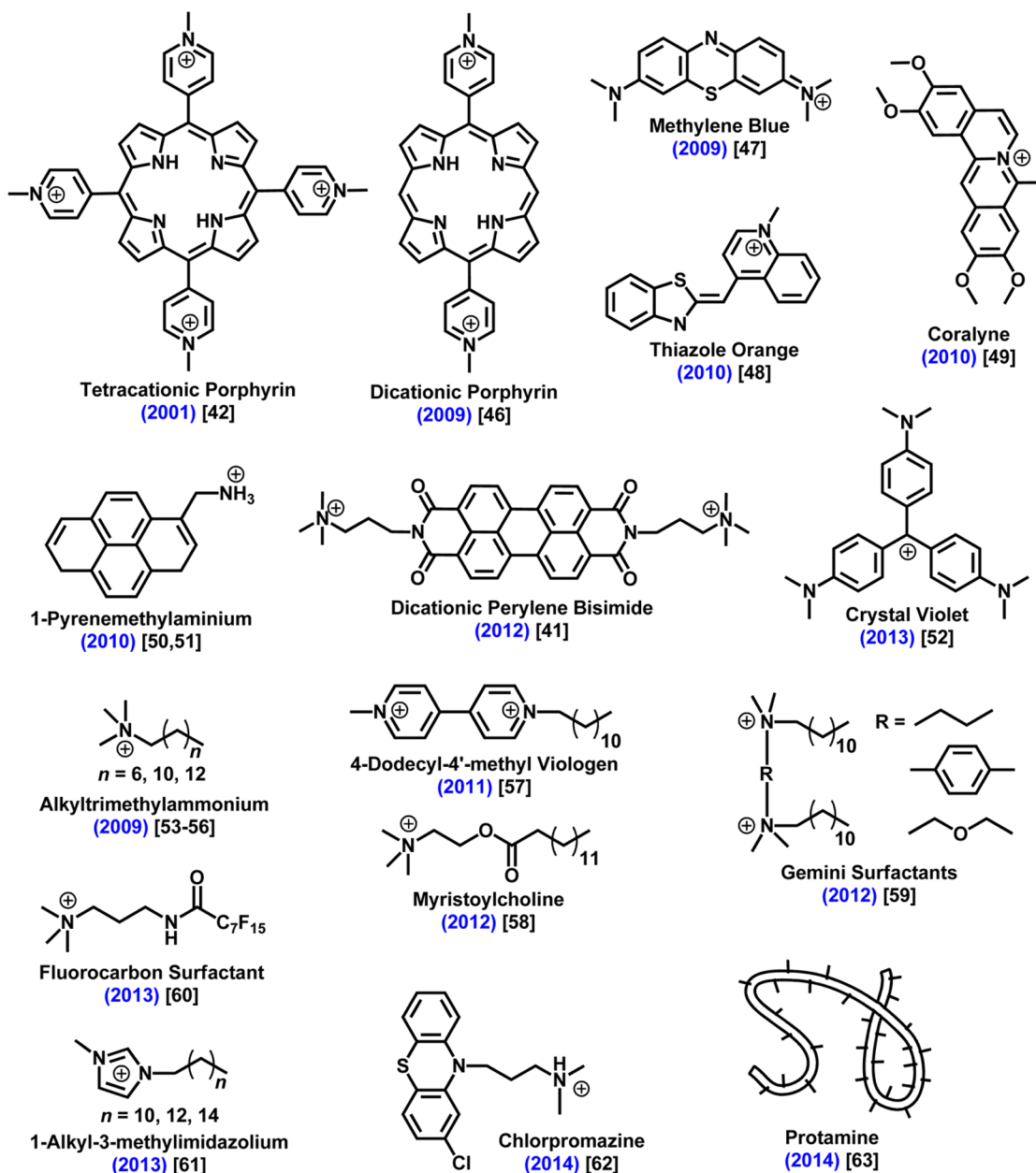
Scheme 6. Chemical Structures of Guest Molecules Used for CIA
