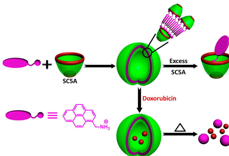
Scheme 8. Construction of SC5A+PMA Supramolecular Binary Vesicles and Temperature-Responsive Drug Release from the Vesicles
