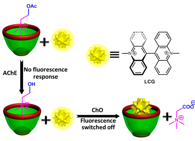
Scheme 3. (Enzyme-Coupled) STA for AChE and ChO Activities, with a Switch-Off Fluorescence Response
