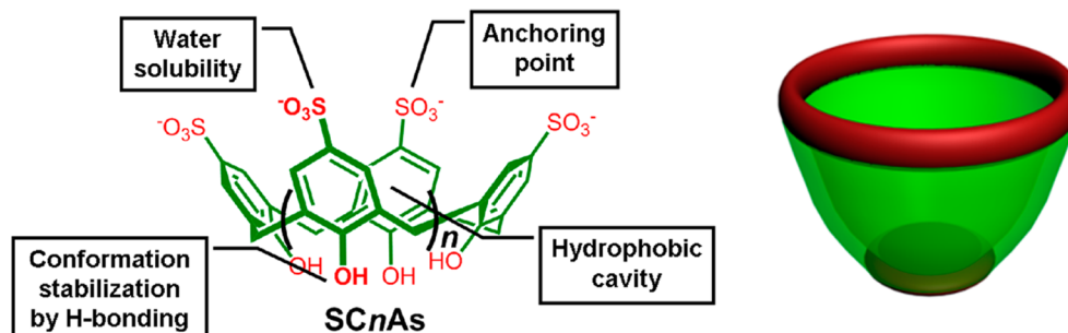
Scheme 1. Structure of SCnAs ( n = 4-8 )
