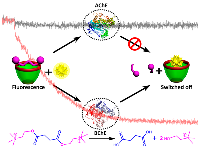
Scheme 4. STA Specific for BChE Activity, with a Switch-Off Fluorescence Response
