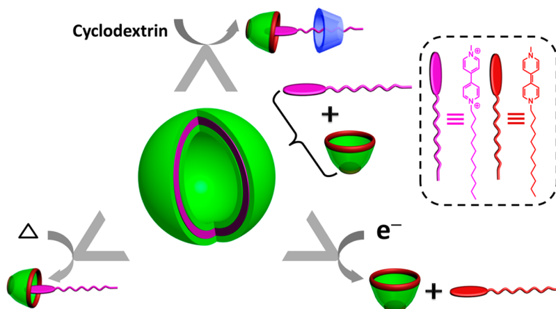
Scheme 10. Enzymatic Responsiveness of Amphiphilic Assemblies of Myristoylcholine Fabricated in the Absence or Presence of SC4A
